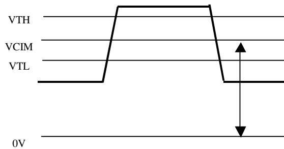
Figure : LVDS Differential Voltage
